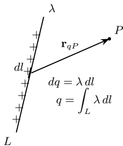
Line charge (b)
